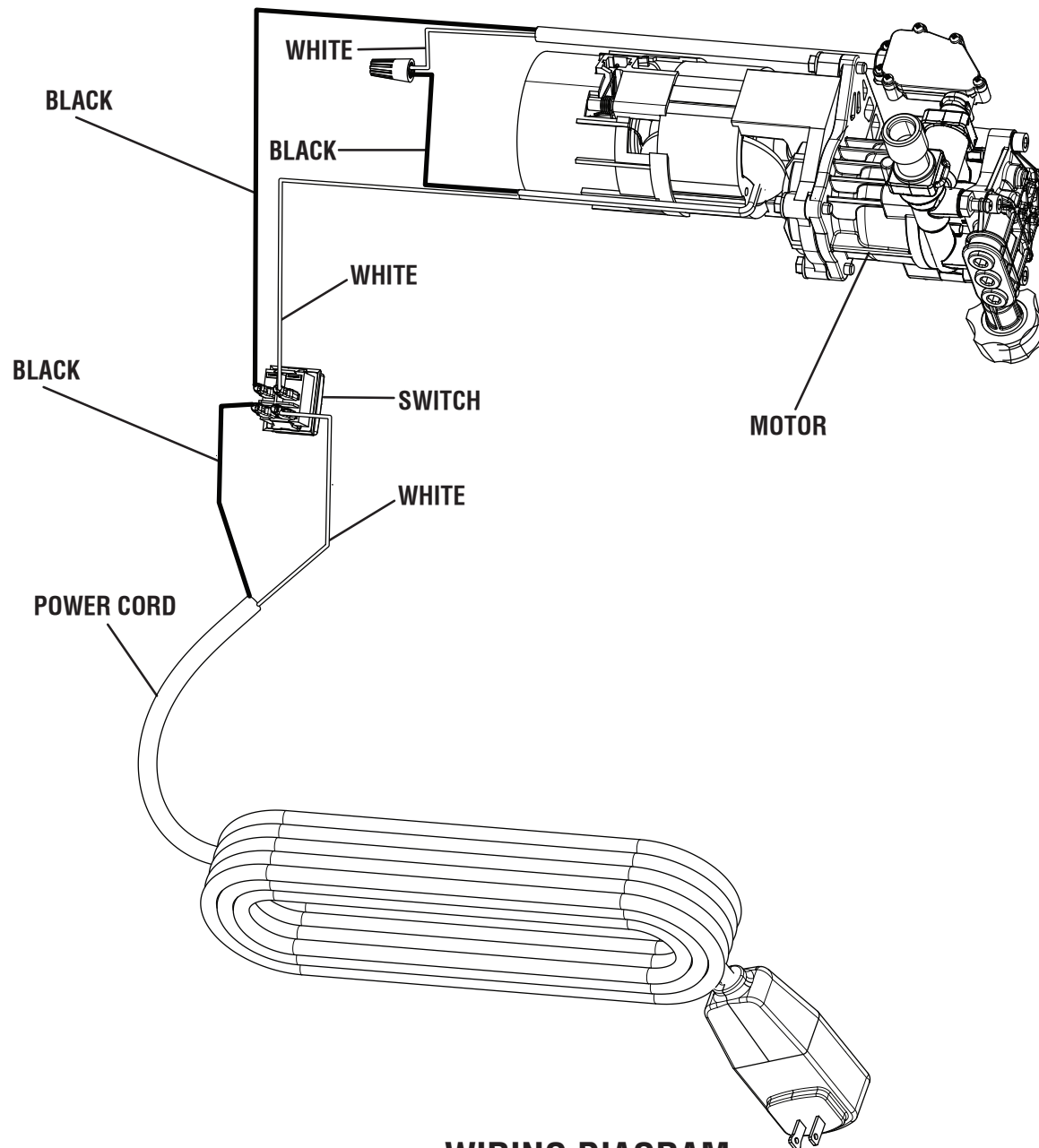
WIRING DIAGRAM
