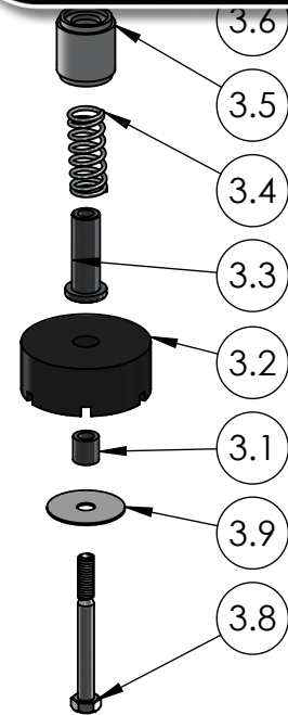
FOOT KIT, WS SERIES SPRING PART NO. 7106951
