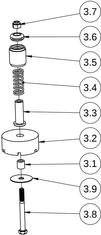
FOOT KIT, WS SERIES SPRING PART NO. 7106951
